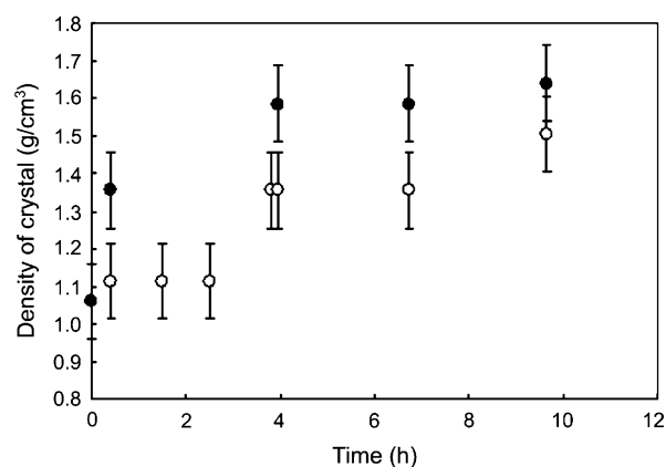
Figure 8. Plot showing the measured density of crystal vs immersion time of the crystal in the DMSO/water (1:1 v/v) (●) and DMSO/CHCl 3 (1:1 v/v) solutions of I_2 (○). I indicate error range of density.
