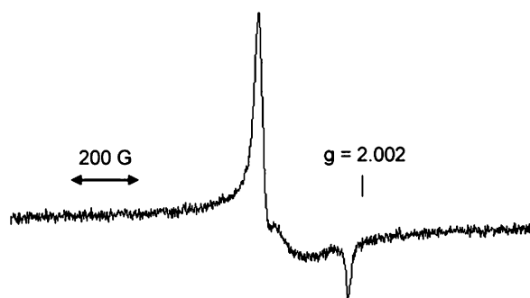
Figure 6. EPR spectrum of 1 (powder sample) measured at room temperature; g_{\parallel} = 2.024 and g_{\perp} = 2.182 .
